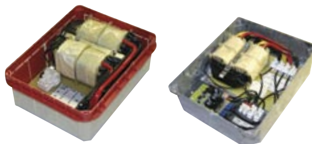
10. Transformer TT5 and TT5-E1 in the electric installation box (box dimensions: 255x205x71mm, further information: page 87)
